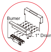
Tube-Fire Heating System
