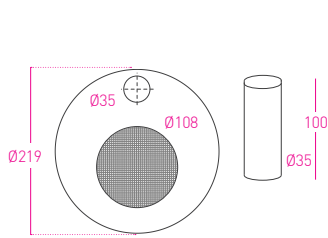
90915 FONT FOR CLASSIC AND ELITE
