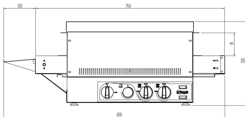
Tampak Samping
