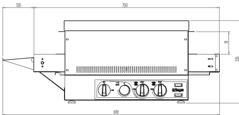
Tampak Samping
