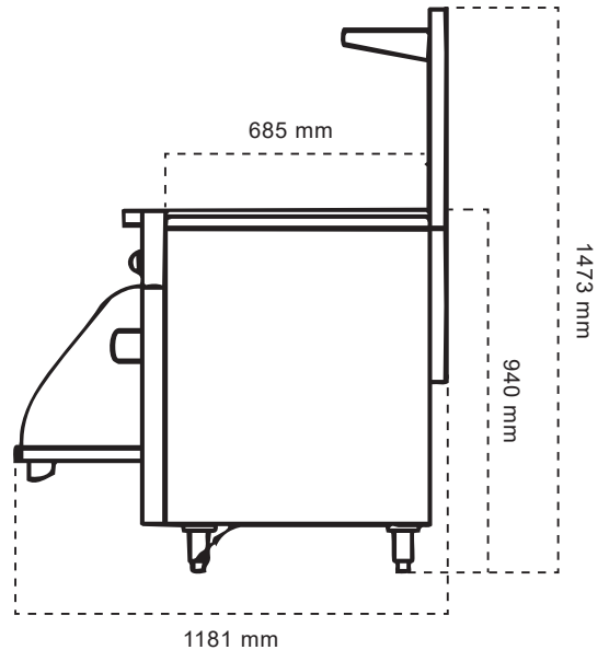
TAMPAK SAMPING
