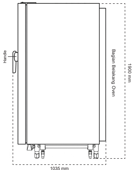
Tampak Samping
