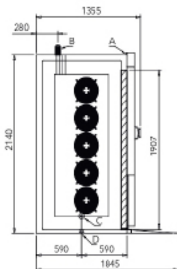
Tampak Samping
