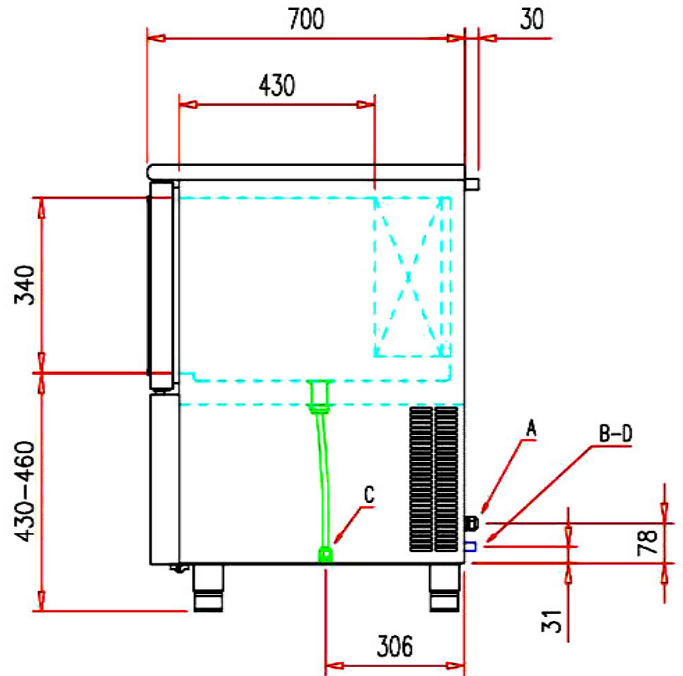
Tampak Samping
