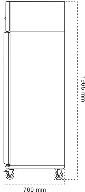
TAMPAK SAMPING
