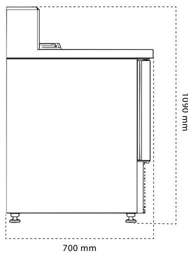
Tampak Samping
