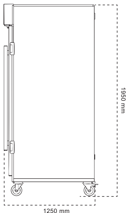
TAMPAK SAMPING
