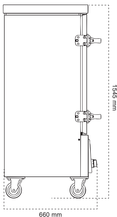
Tampak Samping
