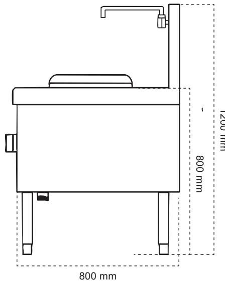
TAMPAK SAMPING
