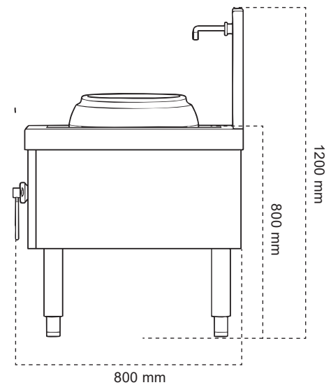
TAMPAK SAMPING
