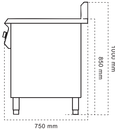
TAMPAK SAMPING
