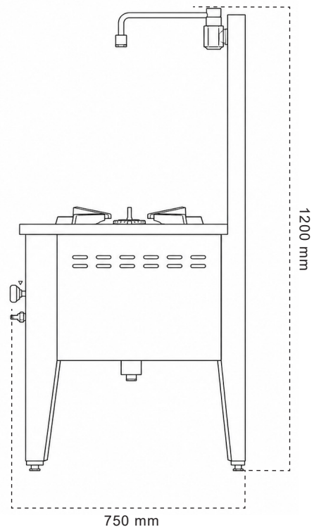
TAMPAK SAMPING
