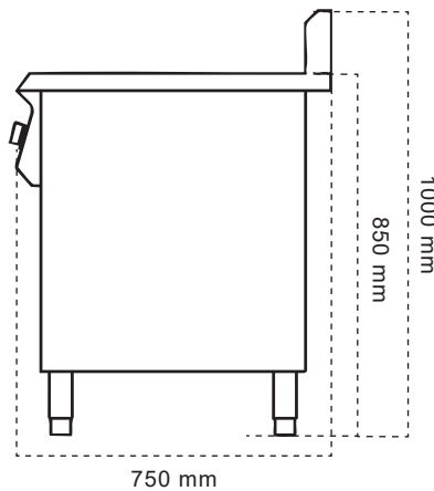
TAMPAK SAMPING
