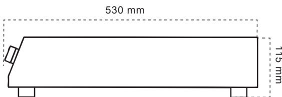
TAMPAK SAMPING
