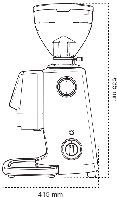
TAMPAK SAMPING
