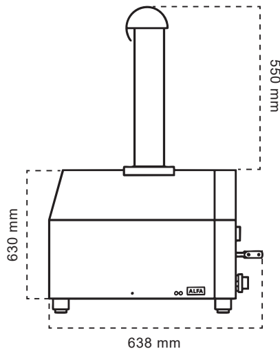
TAMPAK SAMPIING
