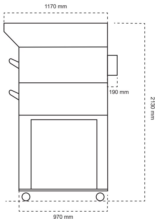
Tampak Samping
