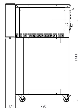
Tampak Samping
