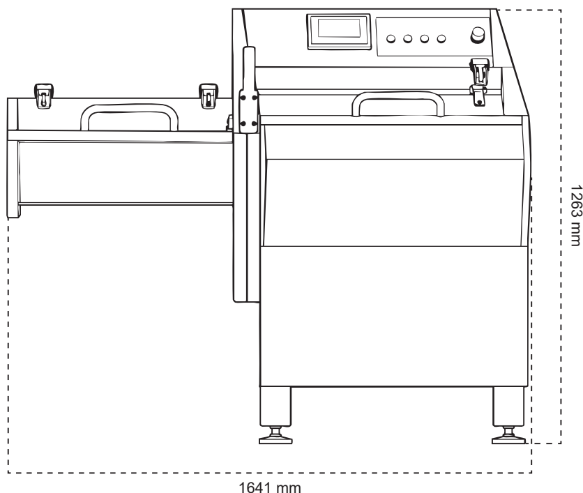
TAMPAK SAMPING
