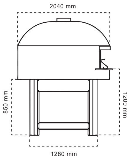
TAMPAK SAMPING
