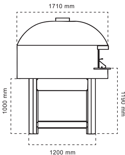
TAMPAK SAMPING
