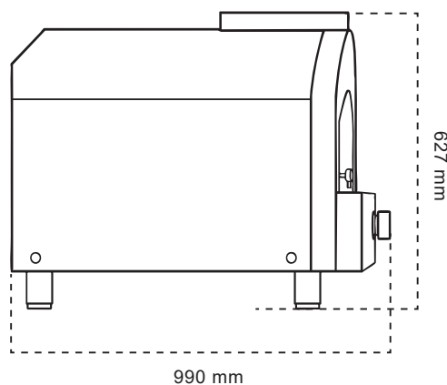
TAMPAK SAMPING
