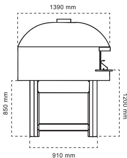
TAMPAK SAMPIING
