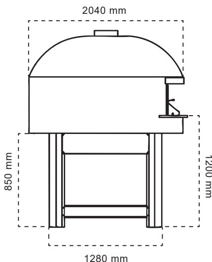
TAMPAK SAMPIING
