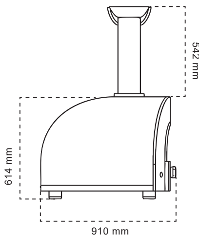
TAMPAK SAMPIING
