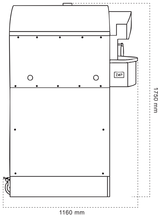
TAMPAK SAMPIING
